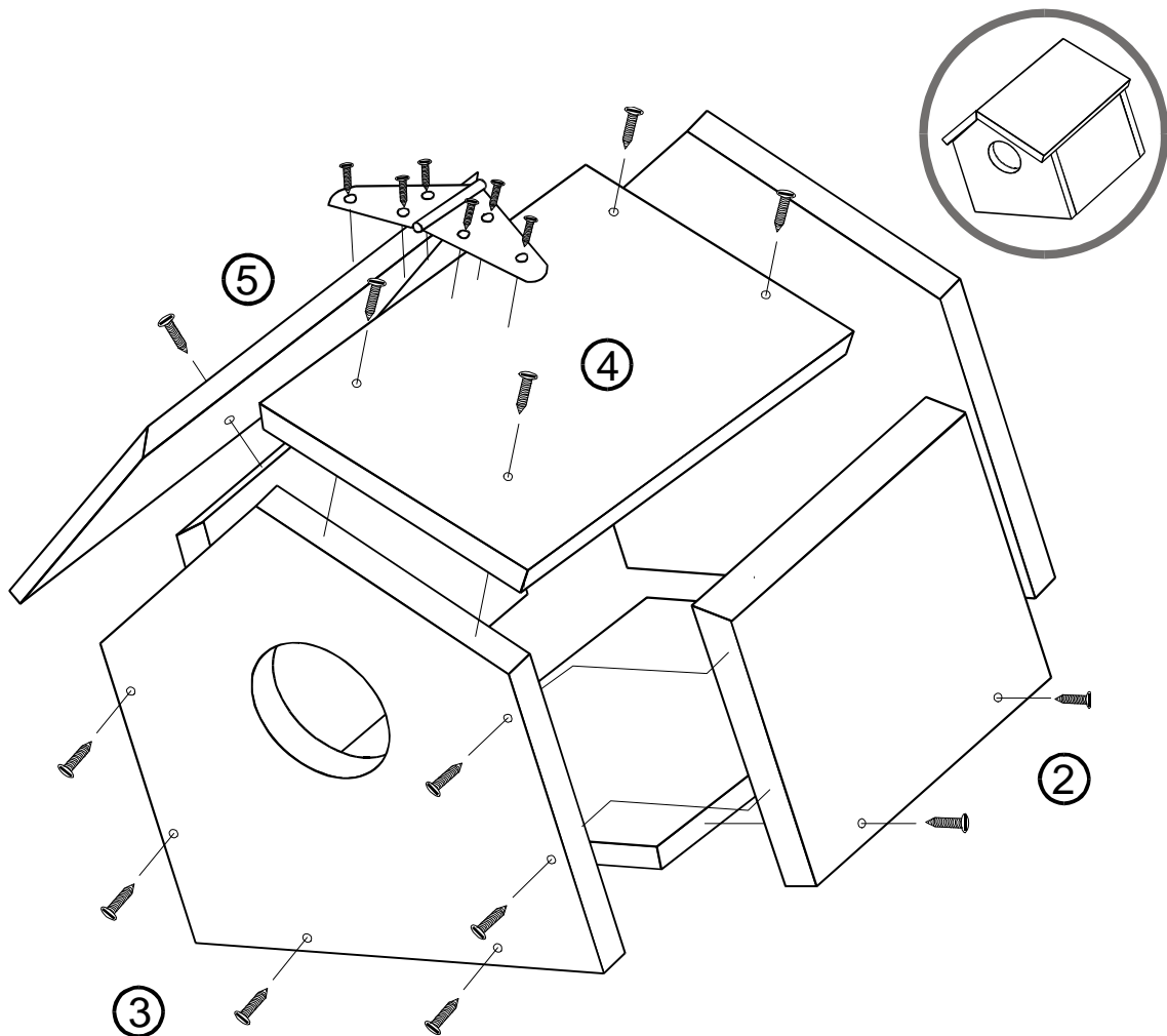
Assembly View
